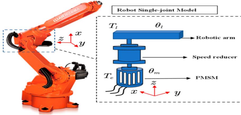
Fig 2: Single joint robot arm.
