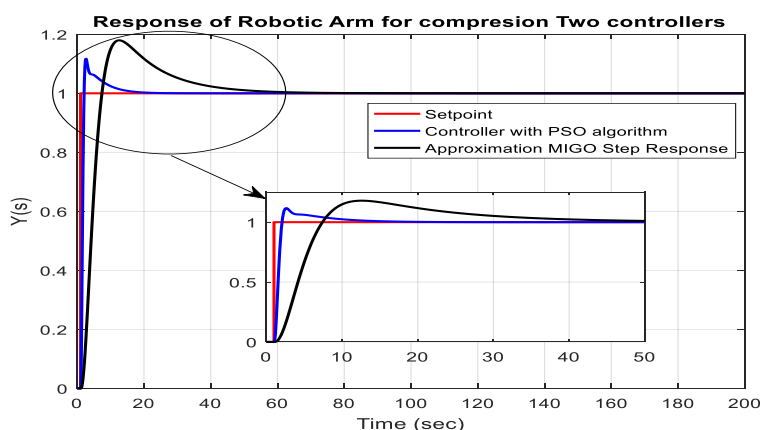
Fig 4: The step response of system using MIGO algorithm and PSO algorithm.
