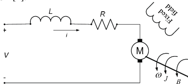
Fig 1: Electromechanical PMDC motor component equivalent representation.
